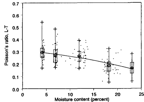
FIG. 16. Relationship of Poisson's ratio in the longitudinal-tangential (LT) direction.
