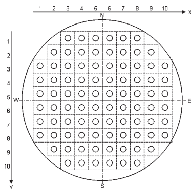
Figure 3. Schematic of hardness mapping grids.
