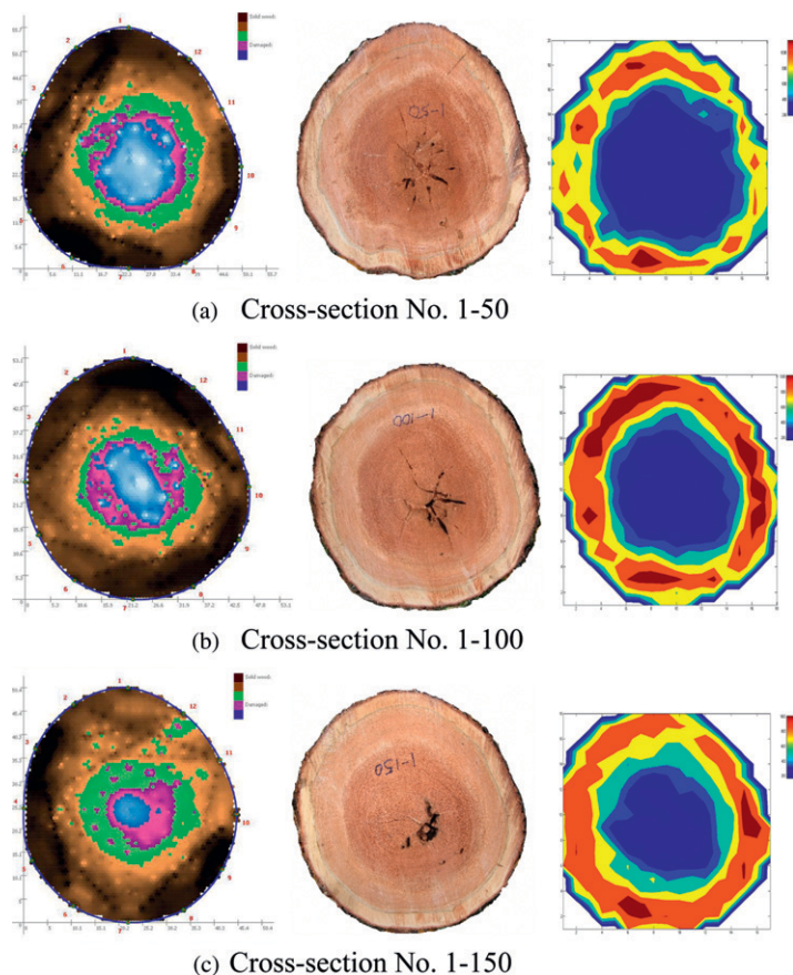
Figure 4. Acoustic tomograms vs photographic images and 2D hardness maps of the discs (tree 1: heartwood decay).
