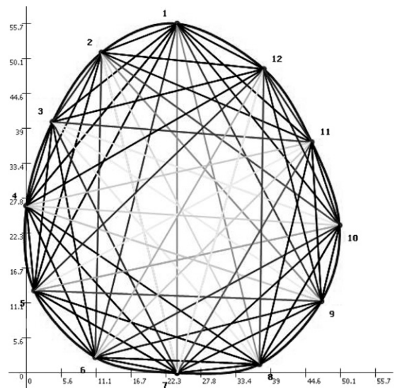
Figure 2. Sensor arrangement and paths of acoustic measurement.
