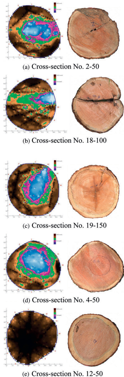
Figure 5. Acoustic tomograms vs photographic images of the discs (trees 2, 18, and 19: internal crack; tree 4: ring shake; tree 12: sound wood with minor defects).
