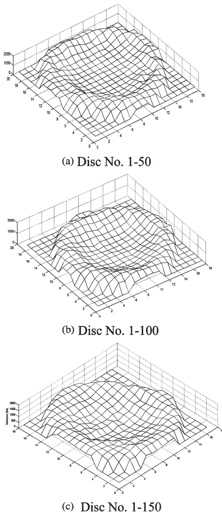
Figure 7. 3D hardness maps of discs with heartwood decay (tree 1).
