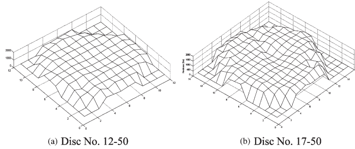
Figure 6. 3D hardness maps of sound discs (trees 12 and 17).
