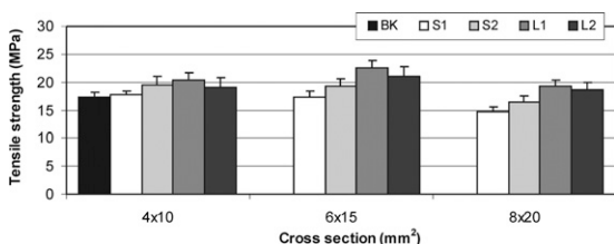
Figure 3. Tensile strength of tested wood-plastic composites (S1, very small; S2, small; L1, large; L2, very large).
