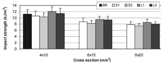
Figure 6. Impact strength of tested wood-plastic composites (S1, very small; S2, small; L1, large; L2, very large).
