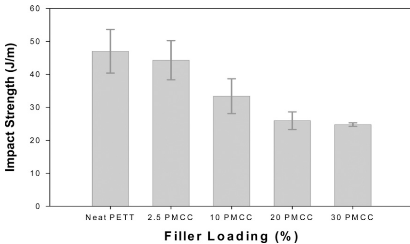
Figure 5. Effect of MCC loading on Izod notched impact strength of PET-PTT blend and MCC-filled composites.
