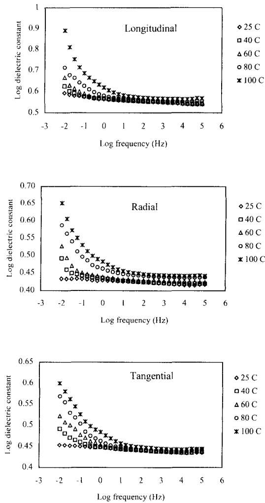
FIG. 1. Dielectric constants for rubber wood at low frequencies, different temperatures, and grain directions.
