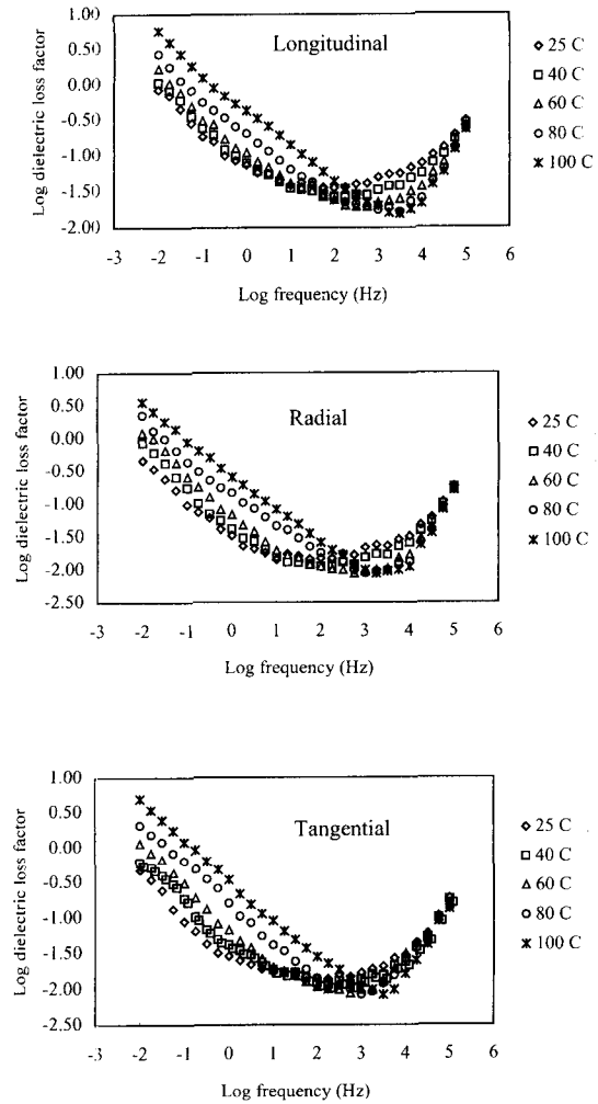
FIG. 2. Dielectric loss factors for rubber wood at low frequencies, different temperatures, and grain directions.
