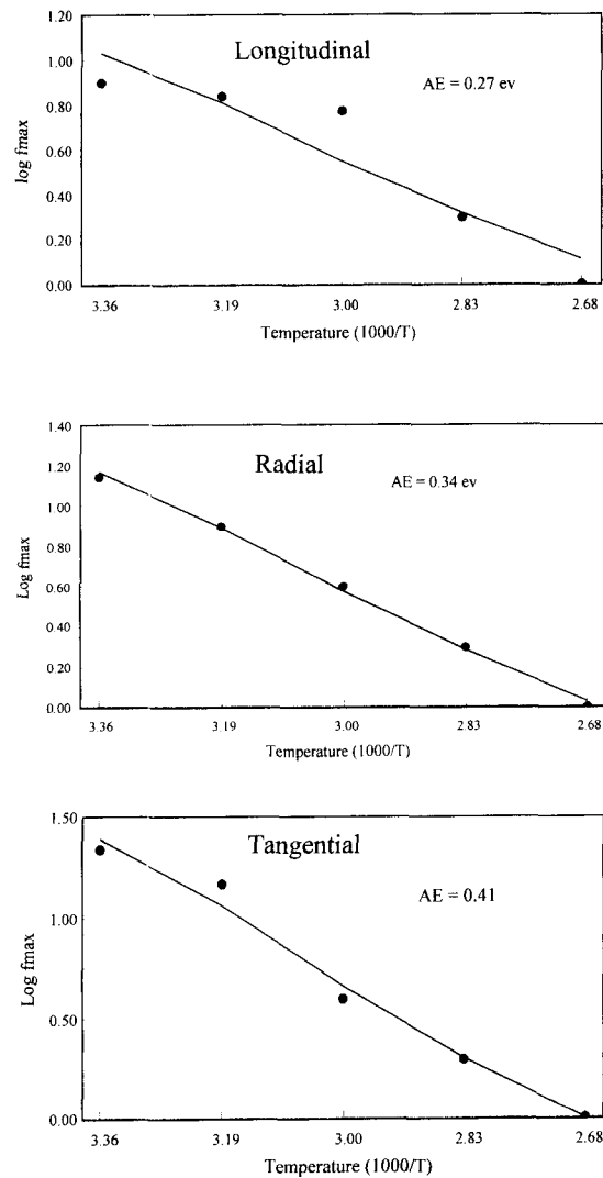
FIG. 4. Activation energies for different grain directions.
