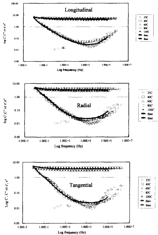
FIG. 3. Normalized data fitted with theoretical value from equivalent circuit for different grain directions.
