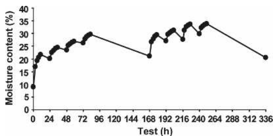
Figure 5. MC of untreated 38-mm \times 140-mm \times 254-mm pine sapwood specimens during exposure to 2 wk of simulated rainfall.
