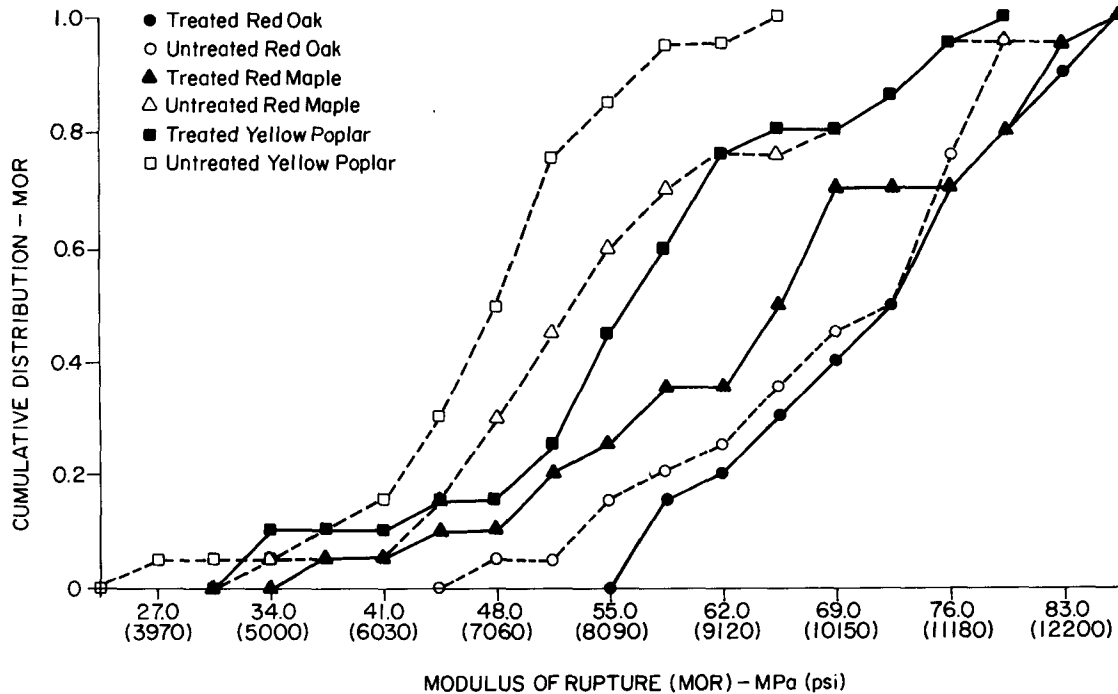
FIG. 4. Cumulative distributions of modulus of rupture for treated and untreated red oak, red maple, and yellow poplar Combination A glulam beams.
