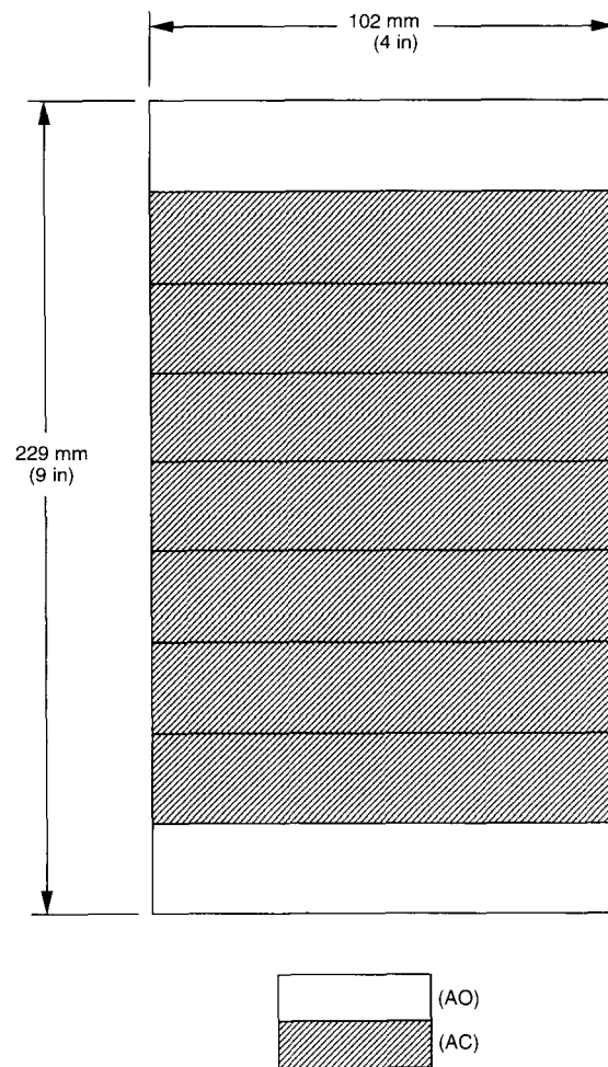
FIG. 1. Layup design for Combination A hardwood glulam.
