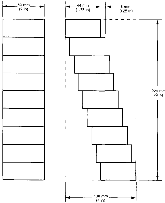
FIG. 3. Typical shear specimen.
