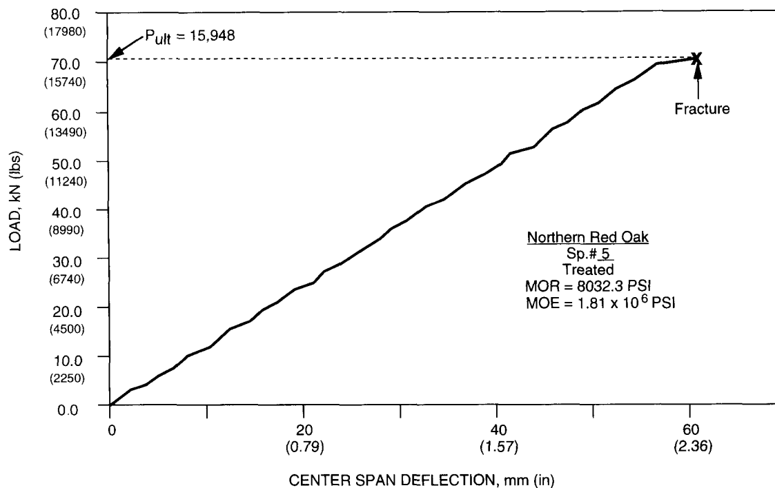
FIG. 2. Typical load vs. deflection curve.
