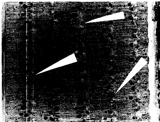
FIG. 5. Micrograph showing some locations of collapsed vessels in white ash—direction of loading is up-down. (20×)
