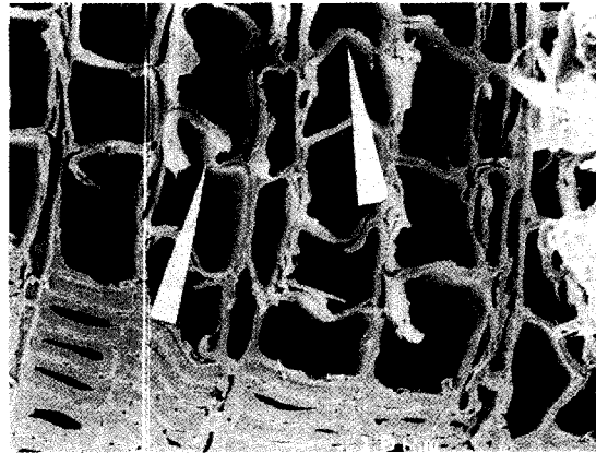
FIG. 7. Micrograph showing bending of tangential cell walls in white spruce under tangential compression—direction of loading is left-right. (400 \times )
