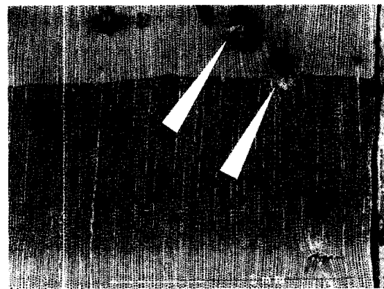
FIG. 10. Micrograph showing localized deformation near resin canals (dark region) in jack pine under tangential compression—direction of loading is left-right. (22 \times )
