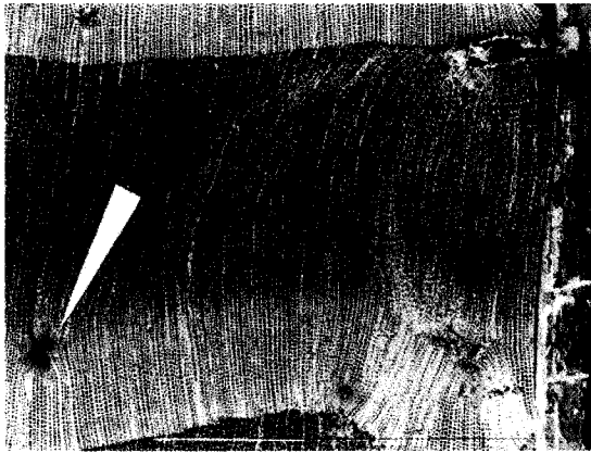
FIG. 8. Micrograph showing initiation of latewood buckling near resin canals in white spruce under tangential compression—direction of loading is left-right. (16 \times )
