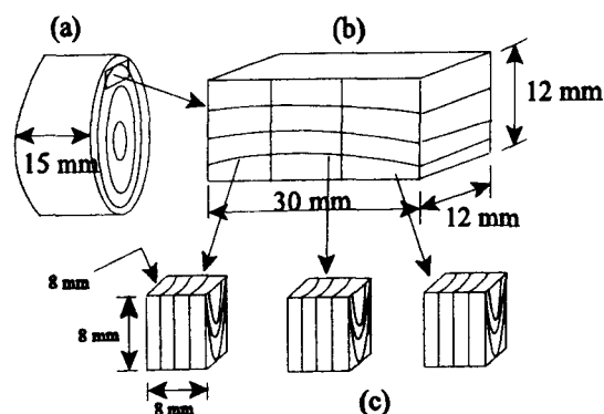
FIG. 1. Preparation of test specimens.
