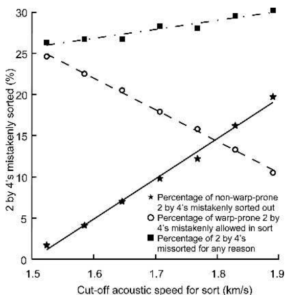
FIG. 4. Relationships between the percentage of ponderosa pine 2 by 4s mistakenly sorted and the cut-off acoustic speed.
