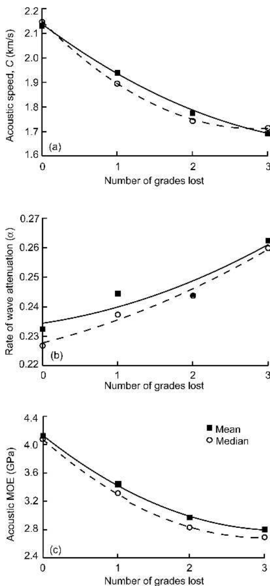
FIG. 3. Relationship between (a) acoustic speed length-wise, (b) rate of wave attenuation, and (c) acoustic modulus of elasticity (MOE) of green ponderosa pine 2 by 4s and the number of grades lost from warp during kiln-drying.
