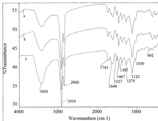
FIG. 2. FT-IR Spectra of extracts F 4 (spectrum a), F 5 (spectrum b), and F 6 (spectrum c).
