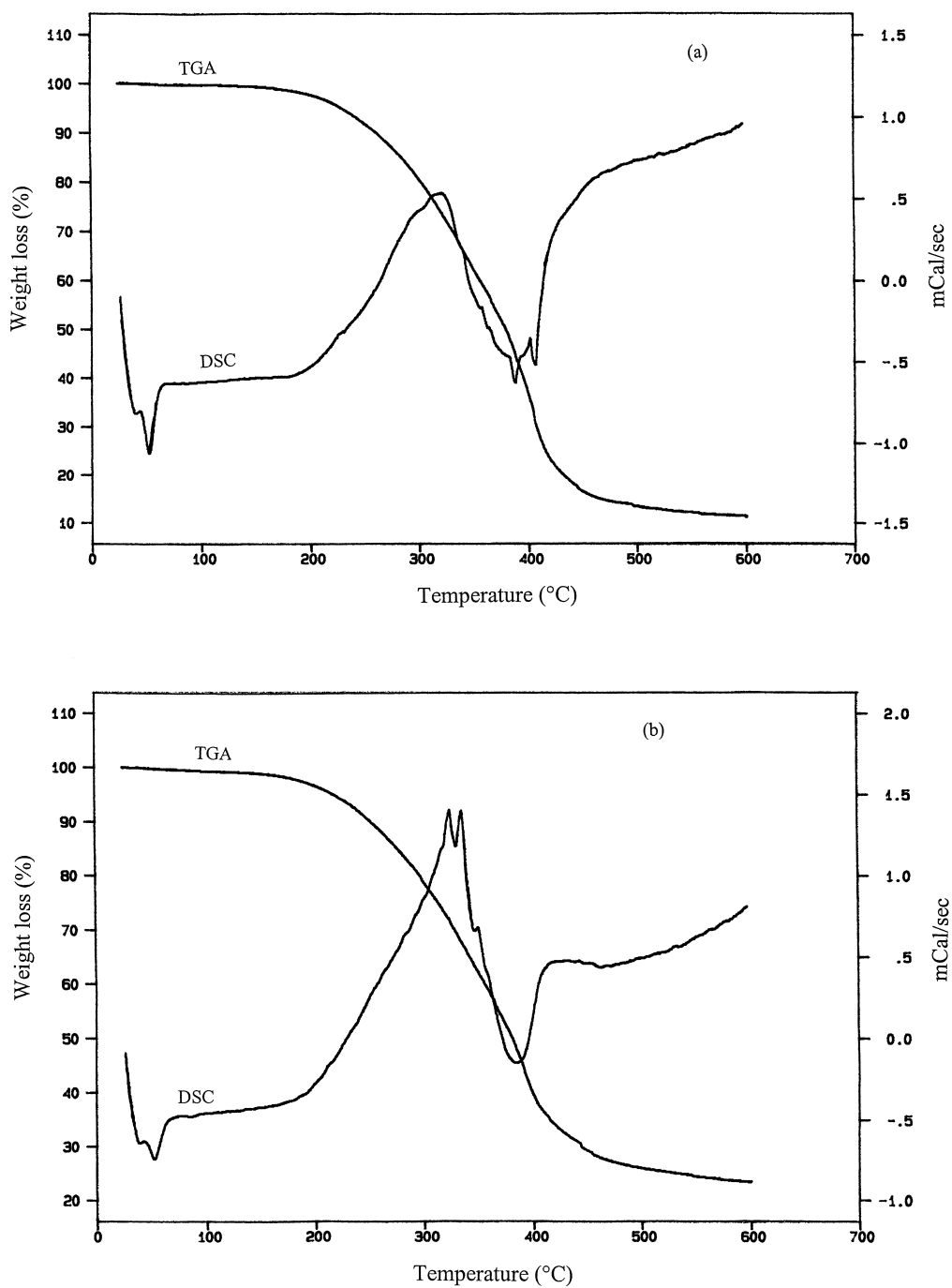
FIG. 5. Thermograms of extracts F 4 (a) and F 6 (b).
