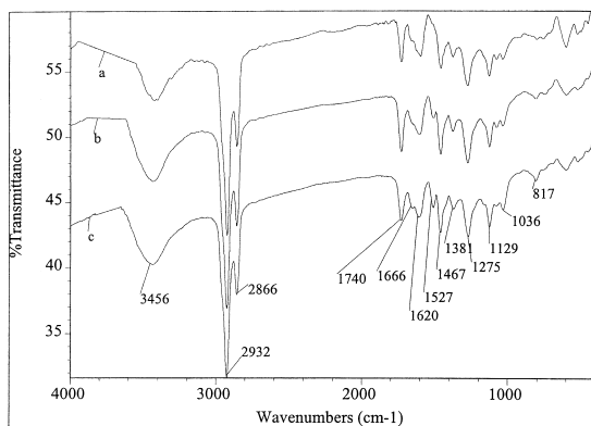
FIG. 1. FT-IR Spectra of extracts F 1 (spectrum a), F 2 (spectrum b), and F 3 (spectrum c).
